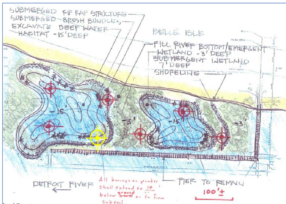
Figure 3 – Planned Geotechnical Boring and Sediment Chemistry Locations
